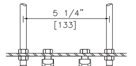
Optional suspension bracket available for 5-1/4" [133] spacing.
