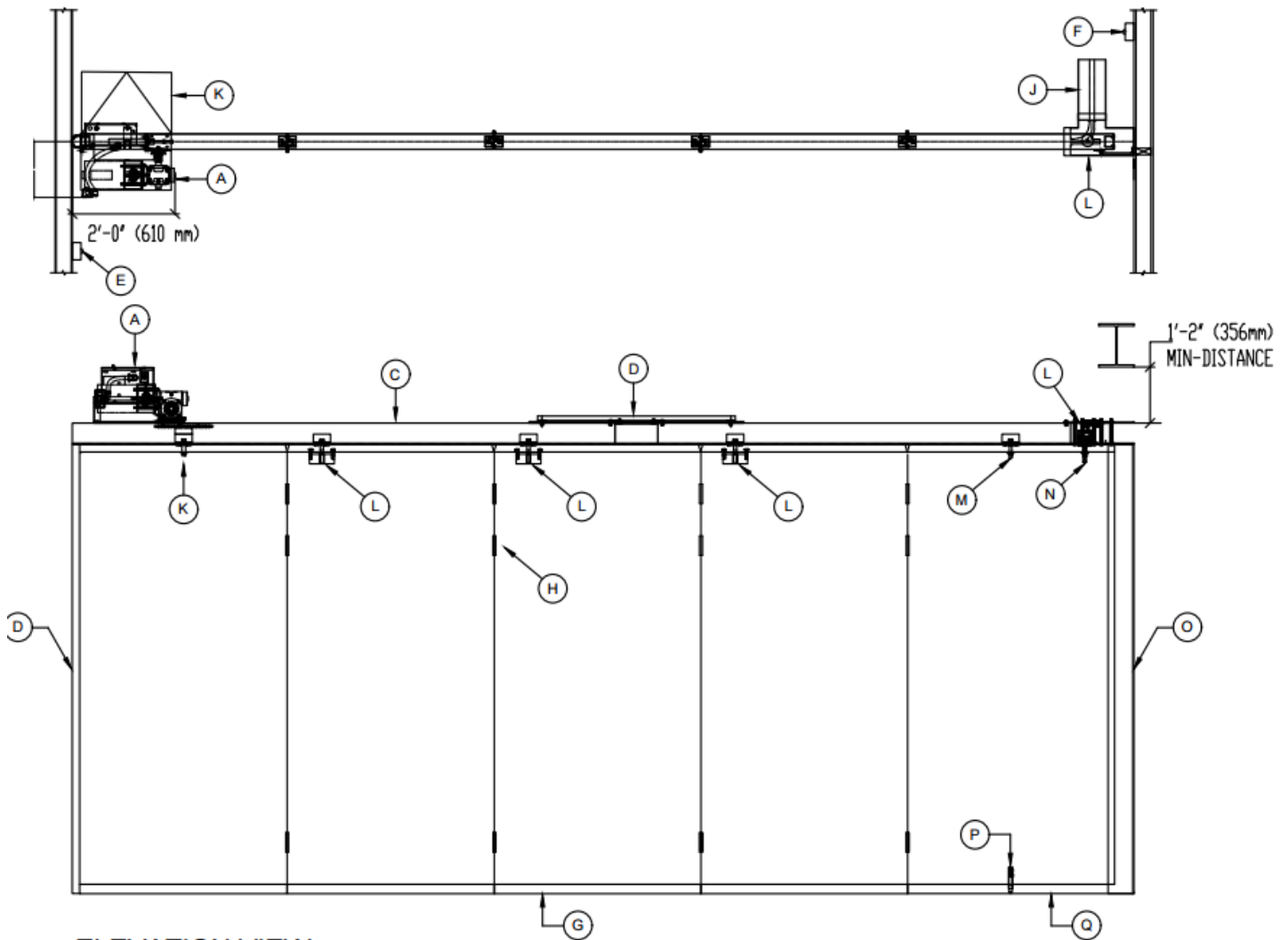
ELEVATION VIEW
