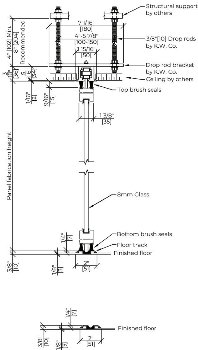
Surface mounted floor track (ADA compliant)
