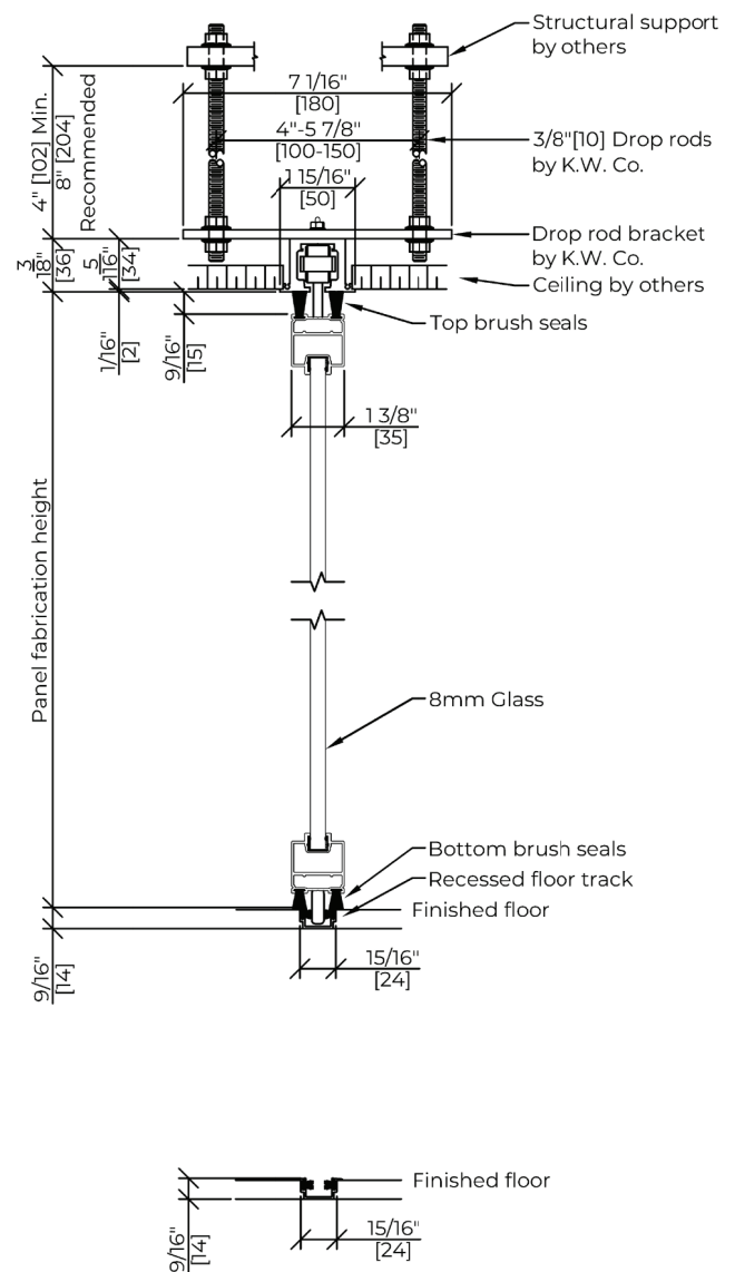
Recessed floor track
