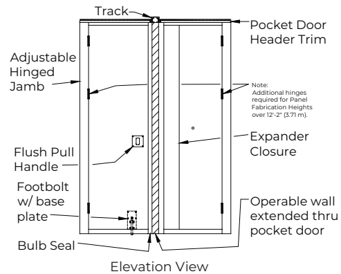
Elevation View
