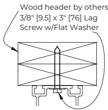
Direct Mount
