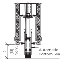
Automatic Bottom Seal
