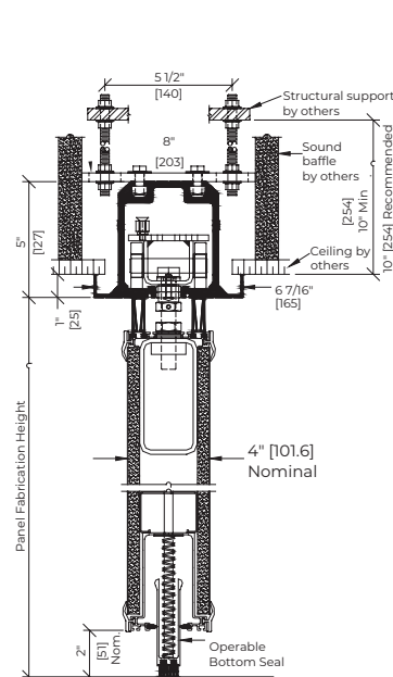
H.D. Curve & Diverter Steel Track and Carrier
