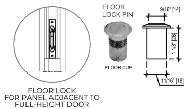
DETAIL AA
