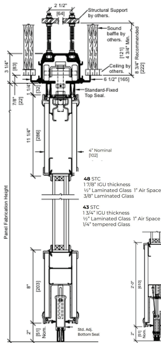
850 Hinged Pairs Aluminum Track & Carriers
