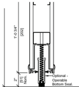
Optional Operable Bottom Seal
