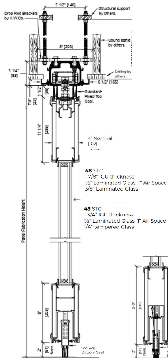
850 Curve & Diverter Aluminum Track and Carrier
